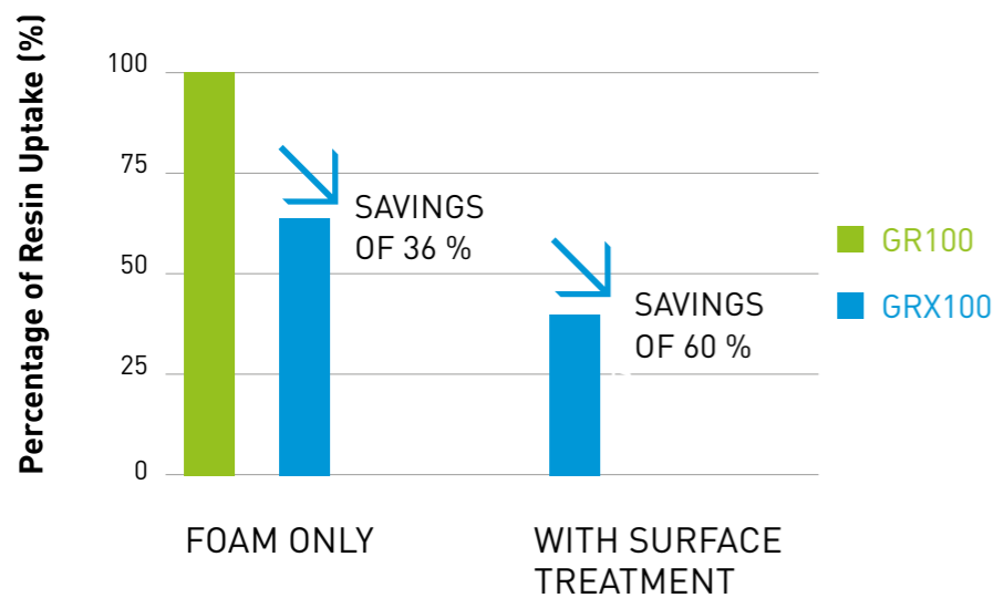
RESIN UPTAKE PERFORMANCE OF ARMAPET STRUCT GR100 VS. GRX100 *
